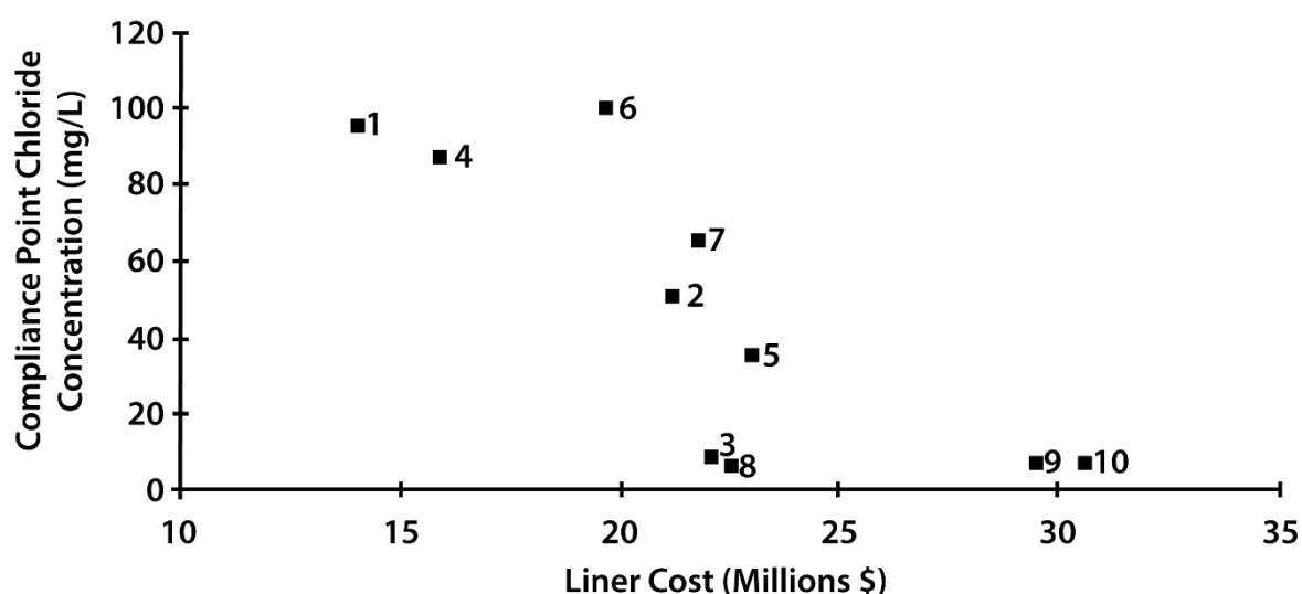
Figure 5 - Expected values of the compliance point chloride concentration versus liner cost expense for different modeling scenarios indicated by numbers next to the data point. The scenarios involve various drainage blanket materials, various clay types and qualities, various leachate tile spacings, and different quality assurance/quality control undertakings.
