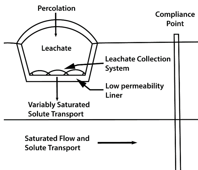
Figure 3 - Schematic of modeling components of exposure pathways impacting the water quality at the point of compliance (McBean, 2019a).
