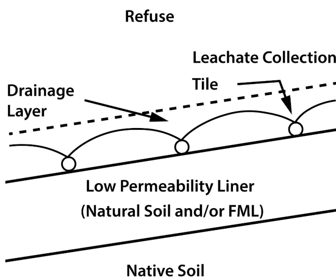
Figure 4 - Leachate collection and liner system (McBean, 2019a).
