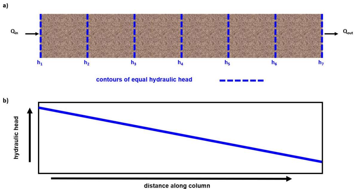
Figure 21 - Steady-state, one-dimensional flow through a homogeneous and isotropic sand column with inflow and outflow openings that are the same diameter as the column: a) the lines of equal hydraulic head (vertical dashed lines) within the saturated sand are perpendicular to the column walls, straight, parallel, and equally spaced, h_1 is the highest head and h_7 the lowest head; and, b) the head distribution is linear.
