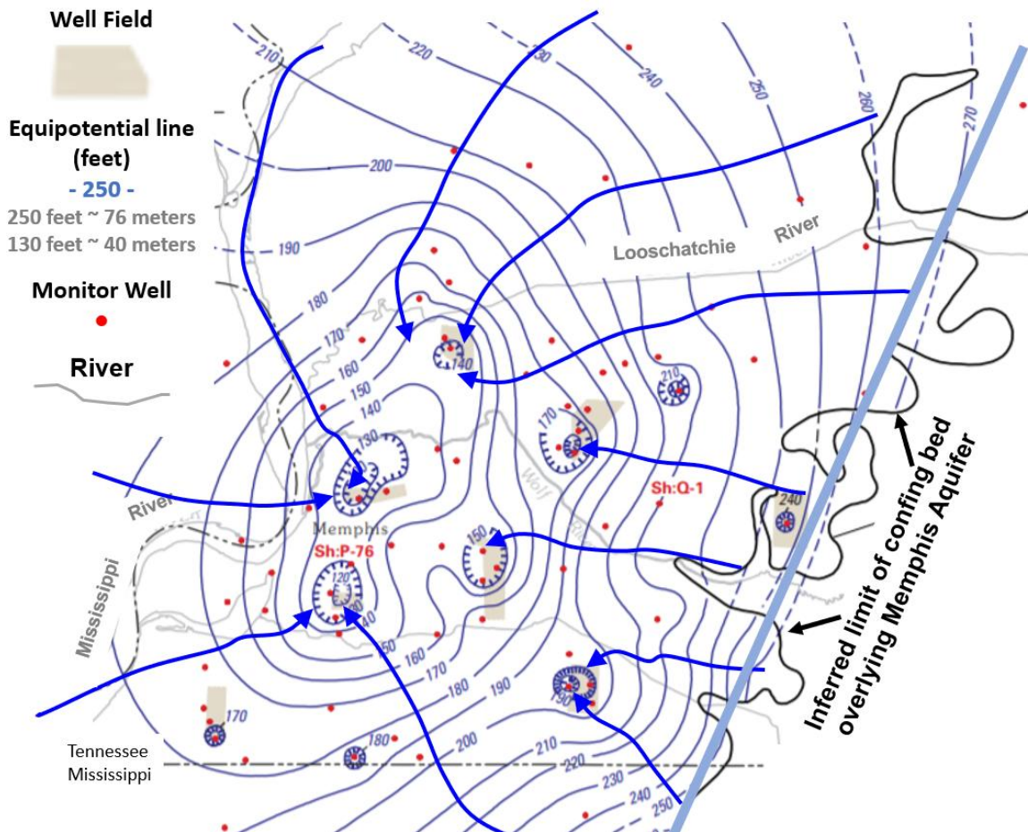
Figure 65 - Potentiometric map (from 1995) of the confined Memphis Sand aquifer in the vicinity of Memphis, TN, USA. Light blue lines are equipotential lines (in feet, divide by 3.28 to convert to meters) interpolated from head data collected at wells (red dots). Dashed lines are inferred. The head distribution shows depressions (areas of lower head) that are indicated by hatched equipotential lines. These areas are associated with long-term pumping of municipal and industrial wells (modified from Taylor and Alley, 2001).
