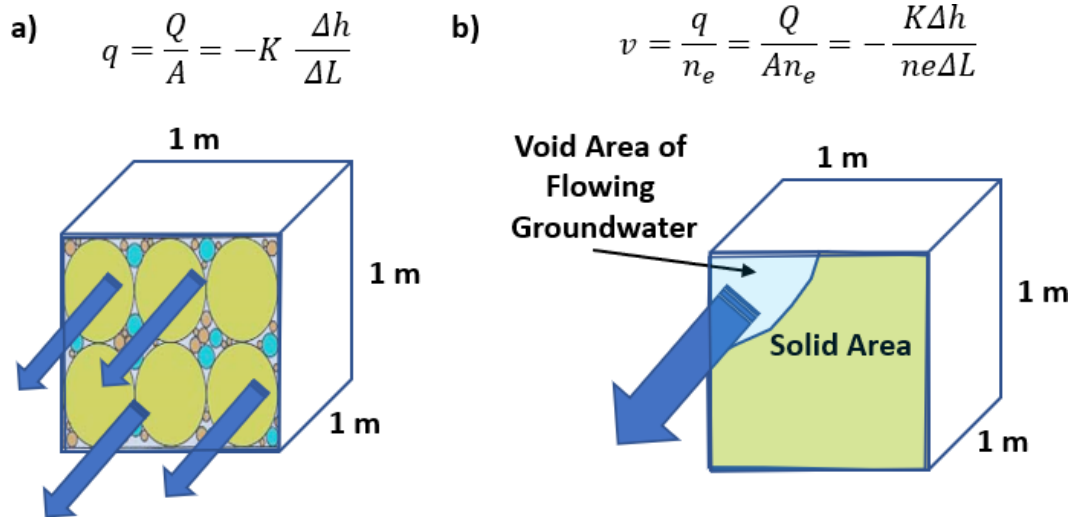
Figure 17 - Conceptualization of specific discharge, q , and average linear velocity, v . a) Specific discharge is the volume per time per unit area of water that leaves the face of the cube (area, including fluid and solids). b) In contrast, the actual rate at which water is flowing through the face is higher than the flux rate because water can only pass through the portion of cross-sectional area that is pore space, (area of pore space = An_e ), where n_e is the effective porosity. The average linear velocity is the flux, q , divided by the porosity, n_e , q/n_e = v .
