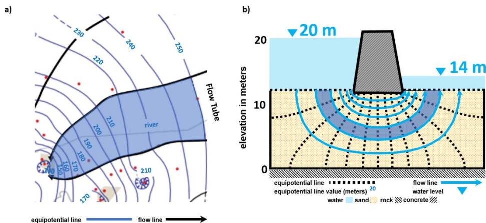
Figure 77 - Schematics of flow nets. Flow tubes are bordered by flowlines. a) A qualitative flow net for which head data at the red dots are hand-contoured and flow lines are drawn at right angles to equipotential lines assuming isotropic and homogeneous conditions. One flow tube is shaded in blue (after Brahana and Borshears, 2001). b) A scaled, hand-drawn flow net of groundwater flow under a dam can be used to quantify flow per unit width of aquifer (Poeter and Hsieh, 2020). A flow tube is shaded in blue.
