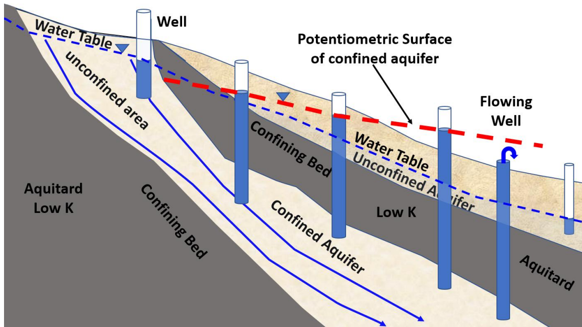
Figure 46 - Schematic of a confined aquifer. The aquifer is located between confining units (aquitards) of low hydraulic conductivity (gray). The recharge area is elevated, and groundwater flow moves into a geologic setting where the confining beds restrict the upward migration of water. Blue arrows indicate the general direction of groundwater flow. The water levels in tightly cased wells rise above the top of the confined aquifer. The surface representing total head in a confined aquifer is referred to as the potentiometric surface (dashed red line). Confined aquifer wells will flow at the land surface without pumping if the potentiometric surface is higher than the top of the well casing as shown by the rightmost confined aquifer well. Confined aquifers can be overlain by other confined aquifers, and, near the surface by an unconfined aquifer.
