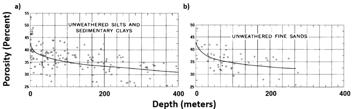
Figure 12 - Examples of decreasing porosity with depth for sedimentary deposits of the South Coastal Basin, CA, USA: a) unweathered silts and sedimentary clays; and, b) unweathered fine sands (after Eckis, 1934; Johnson, 1967).
