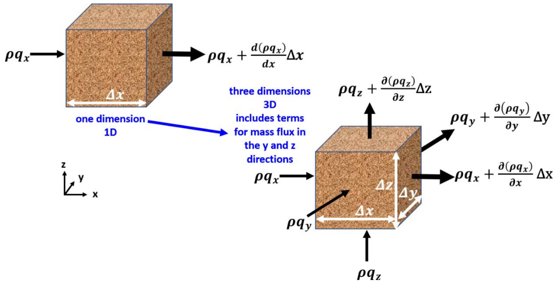
Figure 53 - Representative Elementary Volume showing three-dimensional mass influx and outflux (e.g., \rho q_x ) and an addition or loss of mass flux in the outflow (e.g., (+\frac{\partial \rho q_x}{\partial x} \Delta x) ). This schematic represents confined conditions.
